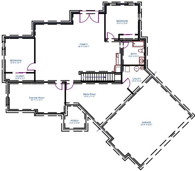
BASEMENT
